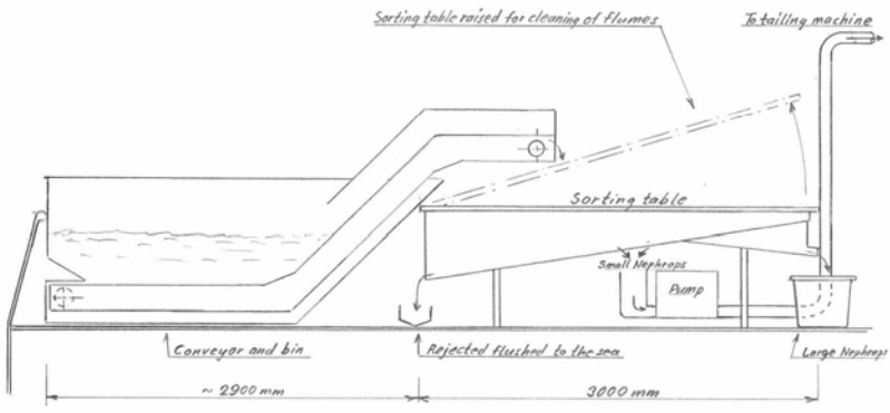
Receiving bin with automatic conveyance to sorting. Pumping of small Nephrops to tailing machine Erik Andersen
